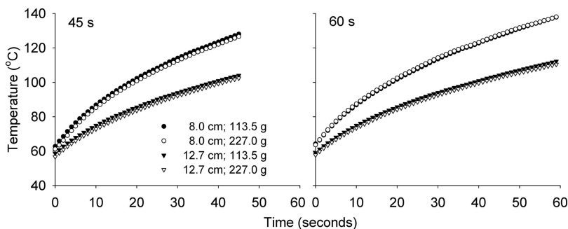
Fig. 1. Generalized time-dependent temperature profile attained with different quantities of wheat exposed at 8.0 and 12.7 cm from the emitter for 45 and 60 s.
